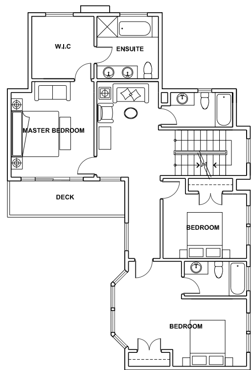
SECOND FLOOR 1186 sq.ft.
